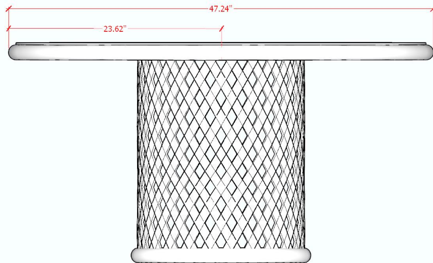
Naples Dining Base w/ 47.24 dia Top
